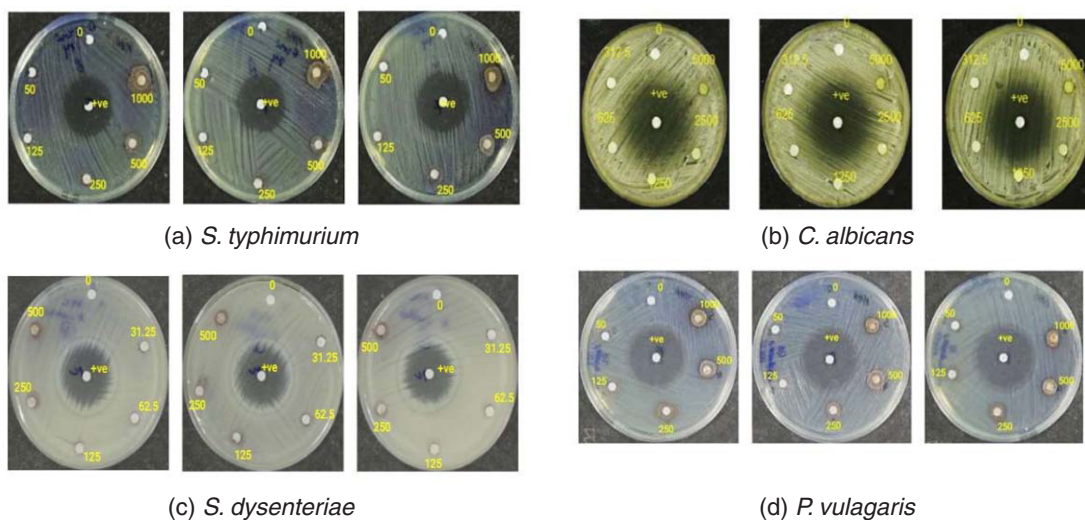
Fig.1. Zone of inhibition (in mm) by Agar disc diffusion method (a) S. typhimurium (b) C. albicans (c) S. dysenteriae (d) P. vulagaris
